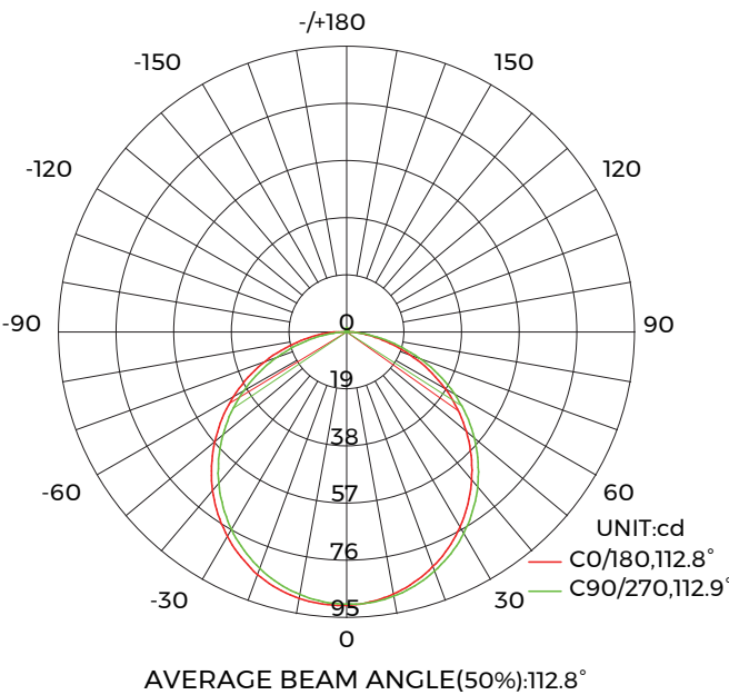
Light distribution
